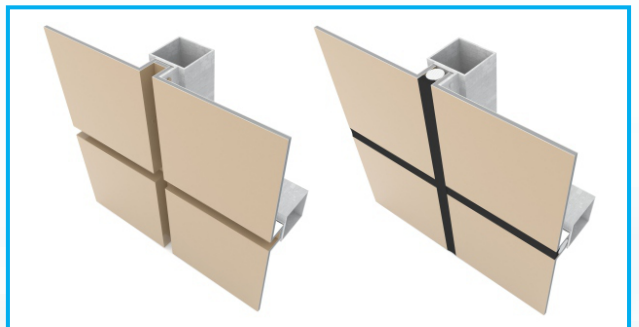
ACP Cladding Pasting & Tray System
